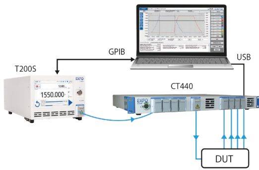
Figure 6. Typical configuration for full band characterization
