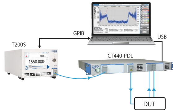
Figure 7. PDL measurement using the CT440-PDL
